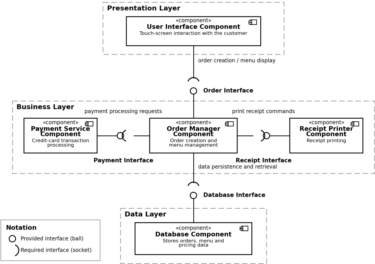
Self-Service Coffee Kiosk System - Layered Architecture
